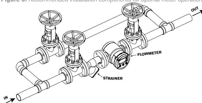
Figure 8: Recommended installation components for optimal meter operation
